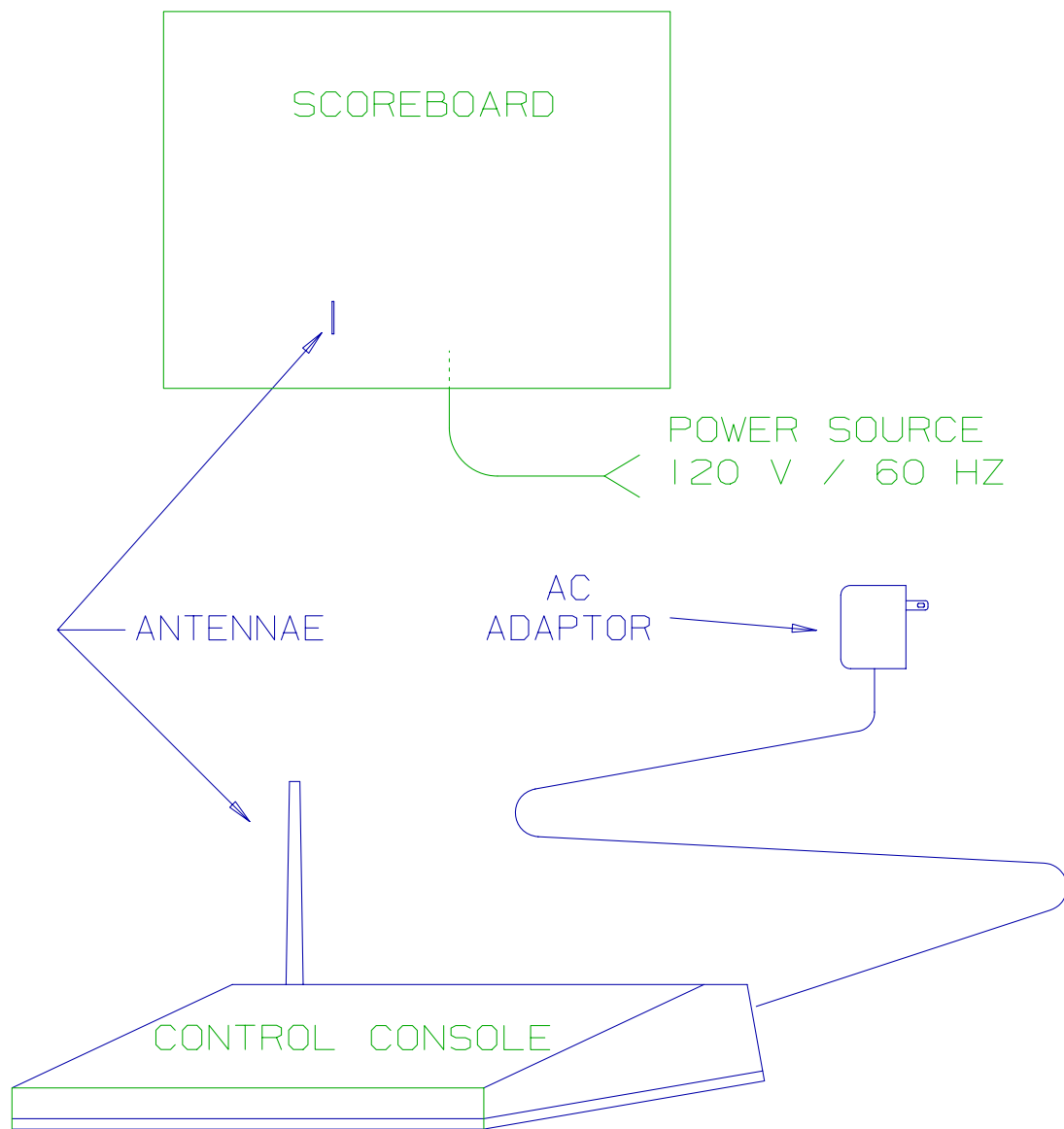
figure 4 SYSTEM LAYOUT
