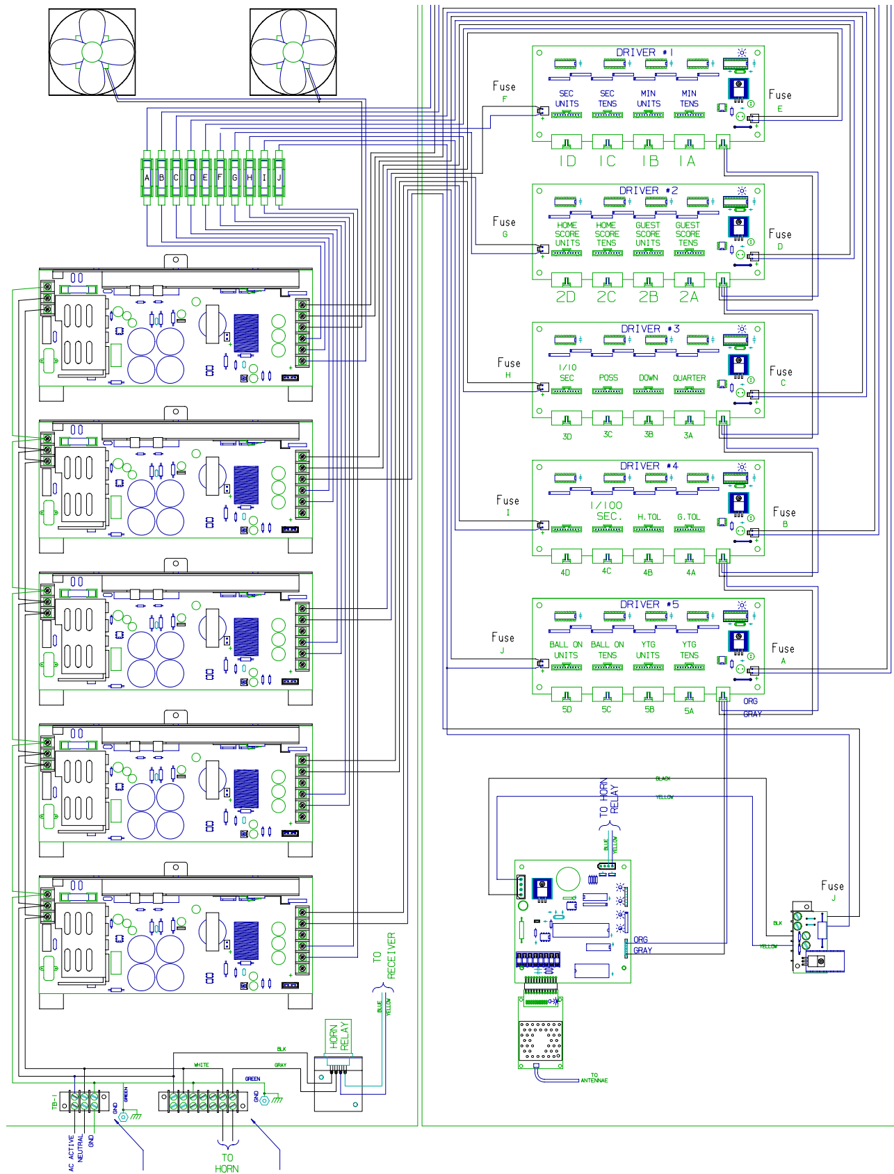
CONTROLLER ASSEMBLY
